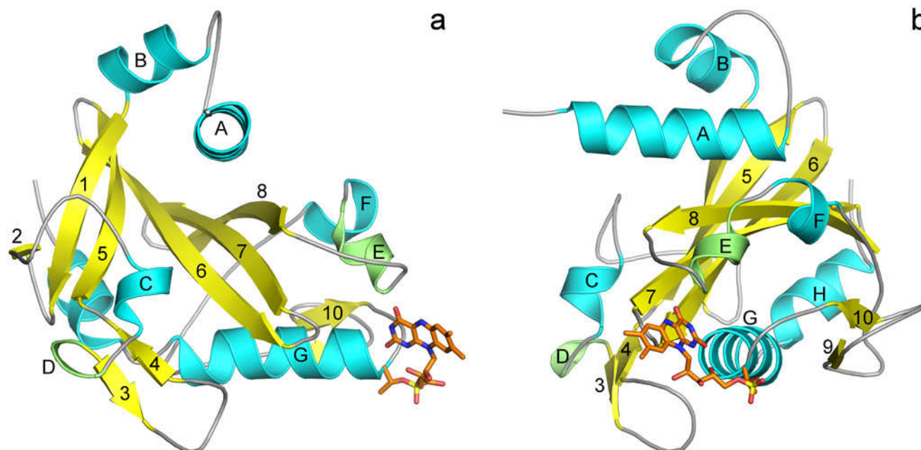
Fig 3. HoloNqrC' structure. (a) and (b)—Overall view with 90°-rotation. Different secondary structure elements are shown in colors: β-sheets in yellow, α-helices in cyan, 3_{10} -helix in green. β-strands and helices are designated with numbers and Latin letters, respectively. Secondary structure was assigned with DSSP [29].
